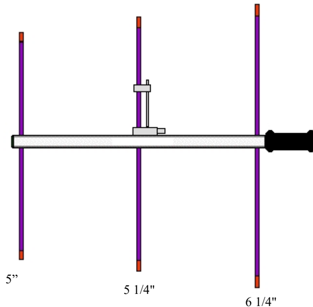
3 Element Portable Antenna for GMRS
